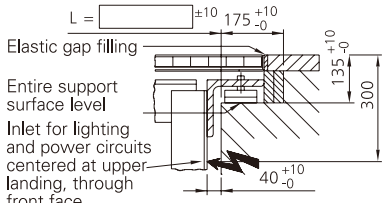
Detail Z
