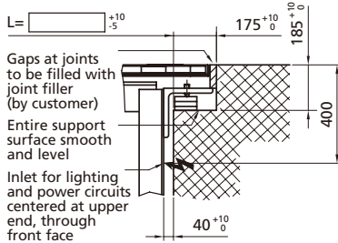
Detail Z
