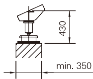
Detail X (1 intermediate support)
